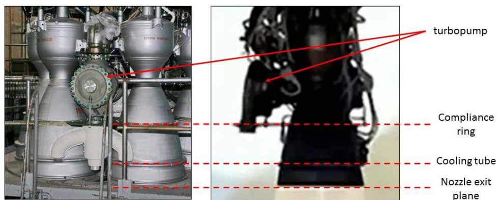
Figure IV Comparison between the RD-250 engine (left) and the engine of the Democratic People’s Republic of Korea (right)
